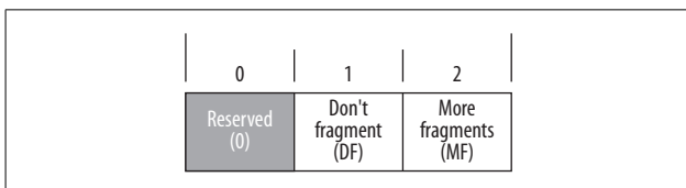
Figure 7. IP version 4 header flags field layout
